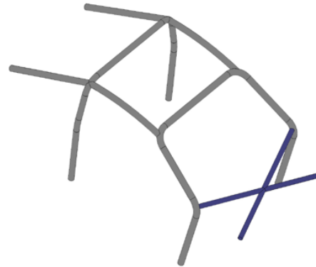
Dessin/Drawing SC-13b
