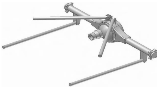
50.5.11 Front suspension
